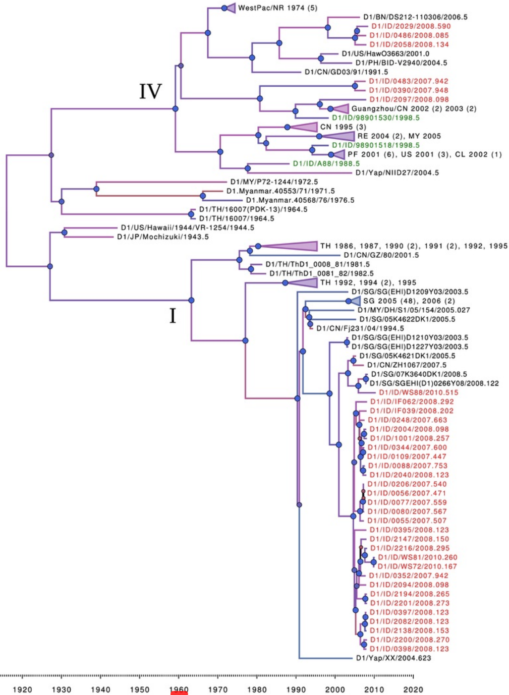
Fig. 1. MCC (Maximum Clade Credibility) phylogenetic tree of DENV-1 Genotype I and Genotype IV. The tree consisted of 35 complete genomes of DENV-1 isolated from Makassar, Indonesia together with their close-distanced genomes available in the GenBank database and was constructed using Bayesian inference as implemented in BEAST. All Makassar isolates were denoted with red labels, while samples from Indonesian cities of Palembang and Jakarta were denoted with green labels. Posterior probabilities of all major branches had values of more than 0.75, indicating the significant of the tree topology. The red line for a branch indicated that the rate of mutation of that particular branch was relatively faster compared to the overall rate of mutation, while the blue line indicated slower rate of mutation. The MCC tree branched into 2 main branches, the genotype IV (upper branch) and I (lower branch). Six of the Makassar isolates grouped into genotype IV, while the rest of Makassar isolates grouped into genotype I. Labels indicating the origin of isolates are as follow: BN (Brunei), CL (Chile), CN (China), ID (Indonesia), JP (Japan), MY (Malaysia), NR (Nauru Island), PF (Polynesian French), PH (Philippines), RE (Reunion Island), SG (Singapore), SC (Seychelles Island), TH (Thailand), and US (United States). (For interpretation of the references to color in this figure legend, the reader is referred to the web version of this article.)
